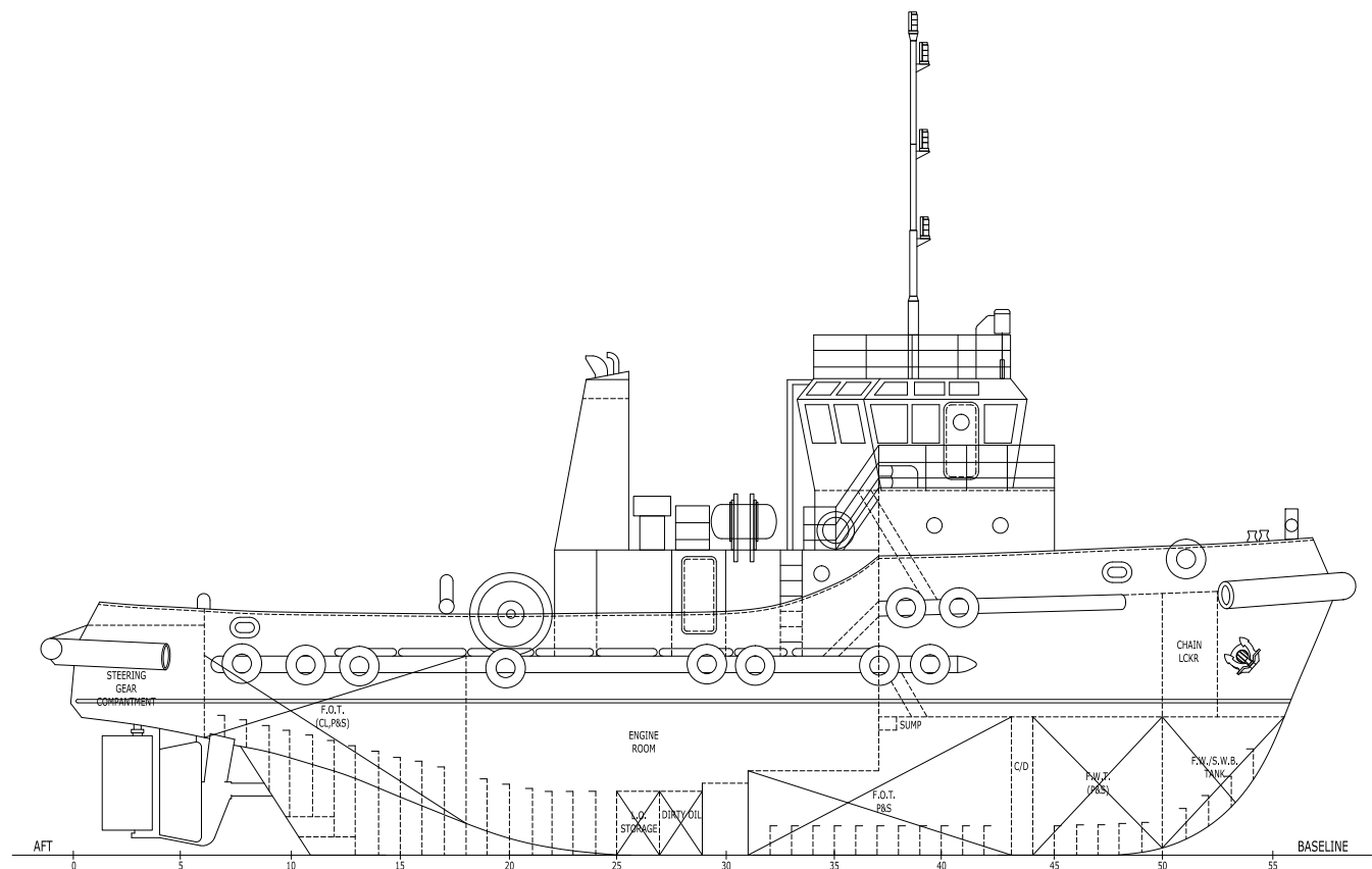
OUTBOARD PROFILE
