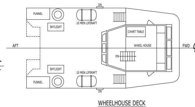
WHEELHOUSE DECK
