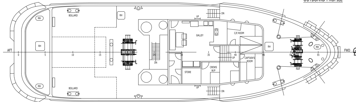
MAIN DECK
