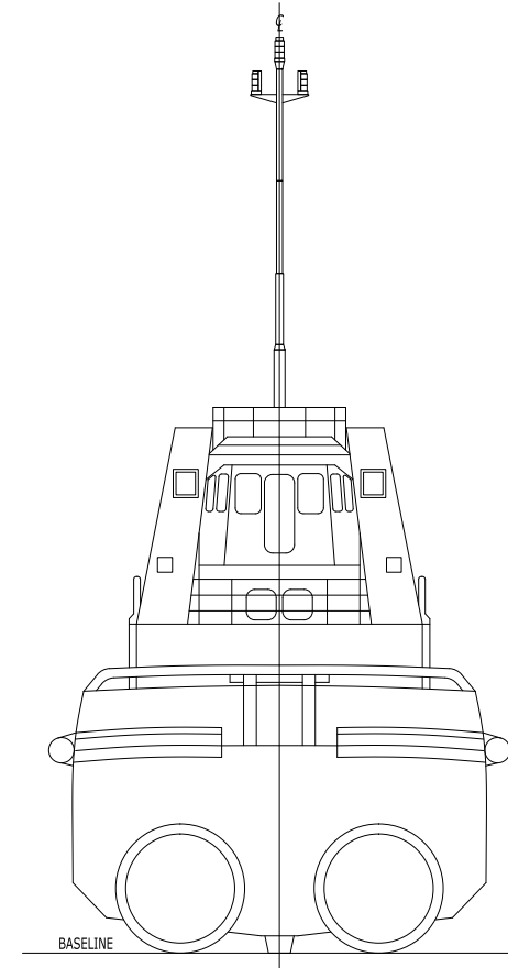
STERN VIEW
